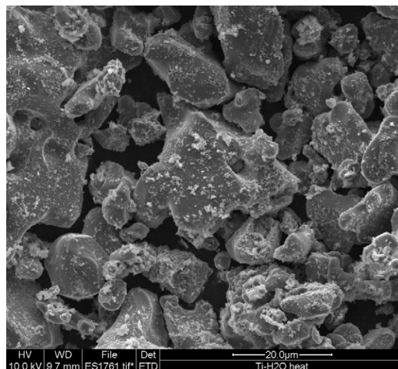
Fig. 5. SEM image of LiCoO 2 coated with TiO 2 aqueous SIC and then calcined. Scale bar is 20 μm.
